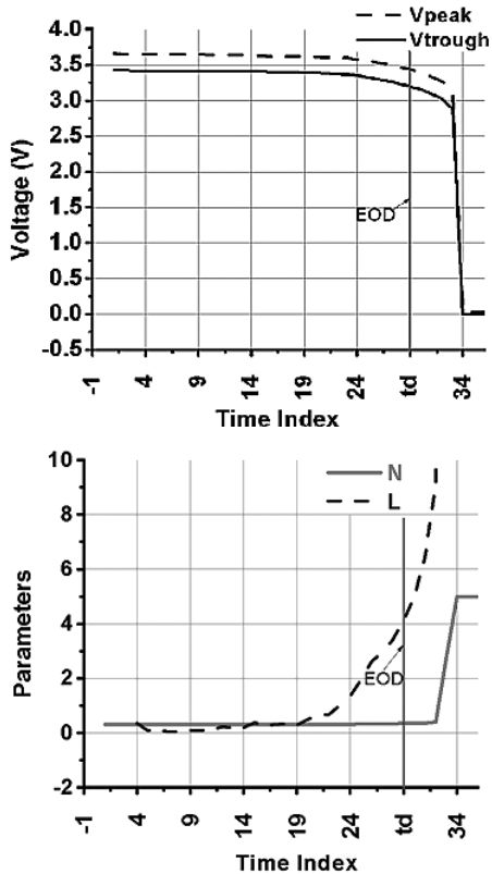
Figure 6. Battery discharging data along with necessary parameters: N and L [(1) and (2)] plotted versus time for a Li-ion battery of 1 cell and 900 mAH capacity. The sampling interval was 2 mins, td is the time index of EOD.
