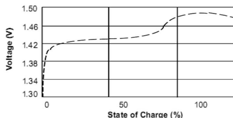
Figure 1. Typical charging profile of a Ni cell [11].
